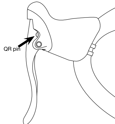
Fig. 4b - To reduce cable tension on the brake caliper for wheel removal, etc., press the cable QR pin fully AWAY from the handlebar stem.
