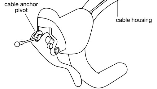
Fig. 2b - Cable Housing Installation
