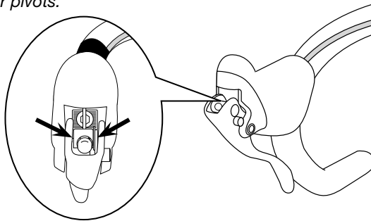
Fig. 5 - To maintain the smooth operation and reduce noise during brake lever operation, periodically lubricate the cable anchor pivots.
